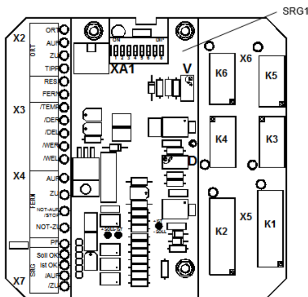
Bild 1: Logic board with positioner SRG1
